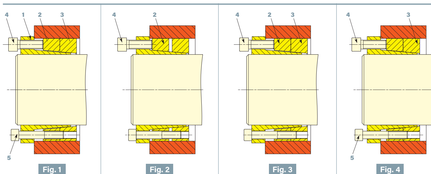
1 Frontal flange - 2 Central thrust ring - 3 Rear thrust ring - 4 Large screws - 5 Small screws
